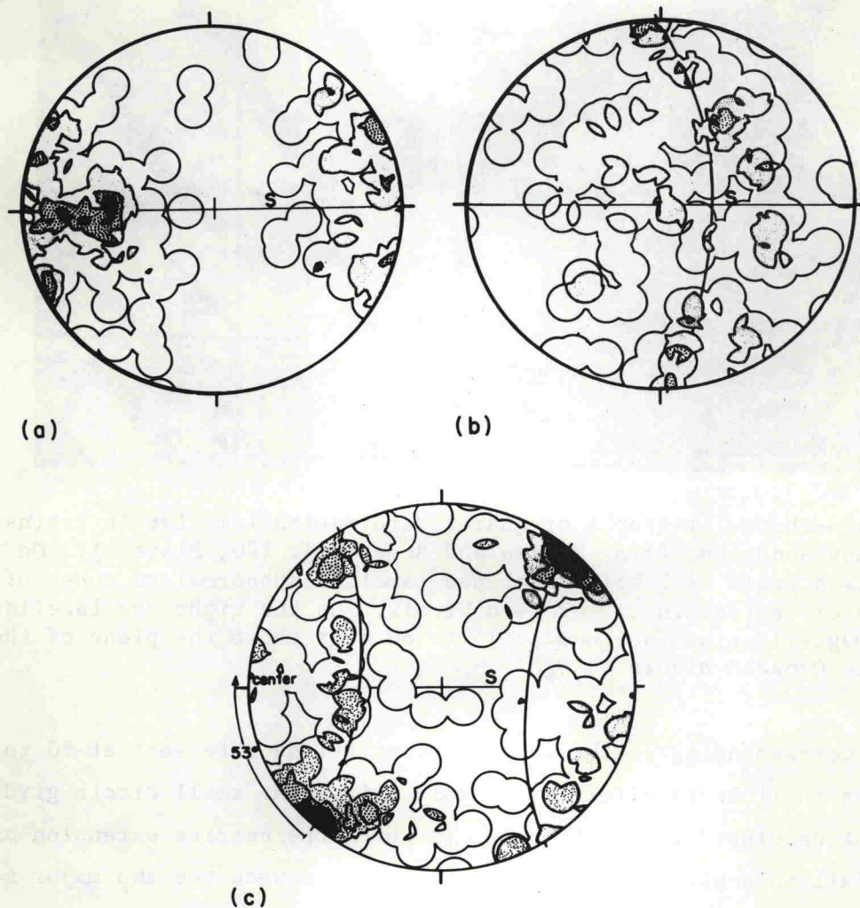
Fig. 43—Diagrams showing orientations of compression and extension axes (a and b) derived from calcite-cement twin lamellae and of quartz deformation lamellae (c) in Oriskany sandstone specimen E2 (from Hansen and Borg, Ref. 120, Figs. 4 and 5). The plane of each diagram is parallel to the ac plane of the fold with the fold axis near the center; s is the bedding plane. (a) 118 compression axes derived from well-developed sets of e twin lamellae in 200 grains. Contours are at 0.9, 2.6, 4.3, and 6.0 per cent per 1 per cent area, 6.8 per cent maximum. (b) 118 extension axes. Contours are at 0.9, 2.6, 4.3, and 6.0 per cent per 1 per cent area. Great circle indicates the trend of the plane containing the extension axes. (c) Normals to 147 deformation lamellae in 400 grains. Contours are at 0.7, 2.1, 3.5, 4.9, and 6.3 per cent per 1 per cent area, 8.4 per cent maximum. The center of the small circle defined by the normals to the lamellae is marked by a dot.
