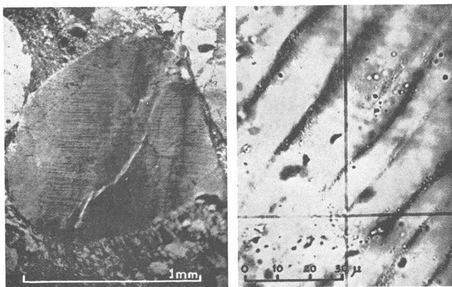
Fig. 42—Photomicrographs of quartz deformation lamellae in grains of Oriskany sandstone (from Hansen and Borg, Ref. 120, Plate 1). On the left is a grain with well-developed lamellae subnormal to zones of undulatory extinction. Crossed Nicols. On the right are lamellae at high magnification inclined at 75 to 80 degrees to the plane of the paper. Crossed Nicols.
